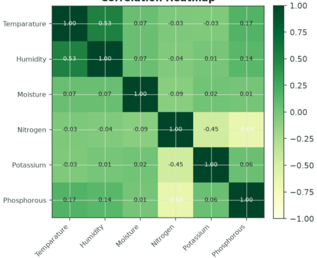
Correlation Heatmap
