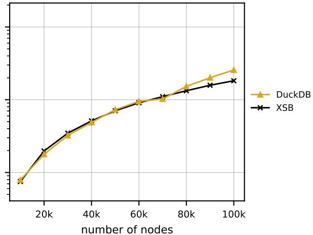
(b) Barabási-Albert: right recursion
