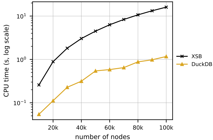
(a) Barabási-Albert: left recursion
