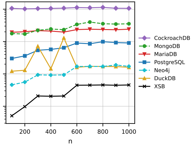
(b) BinTree: right recursion
