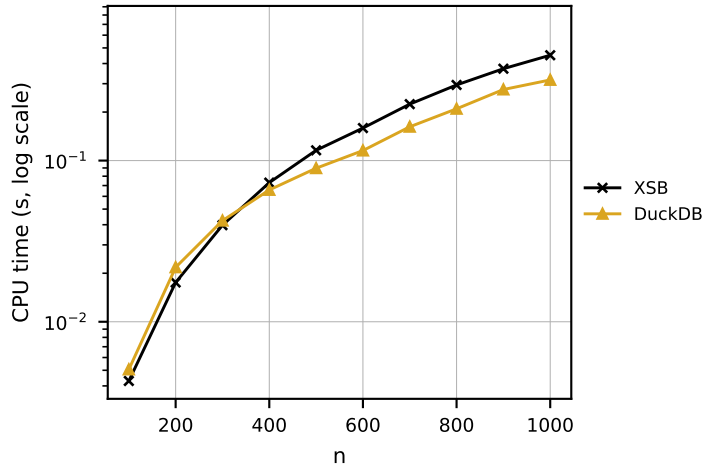
(a) CycExtra: left recursion
