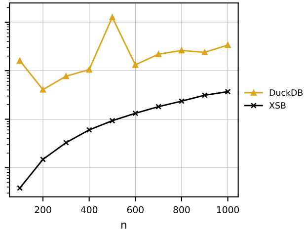
(b) Path: right recursion
