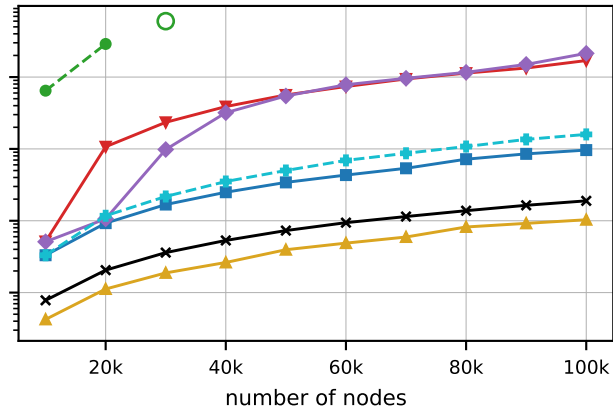
Barabási-Albert: right recursion
