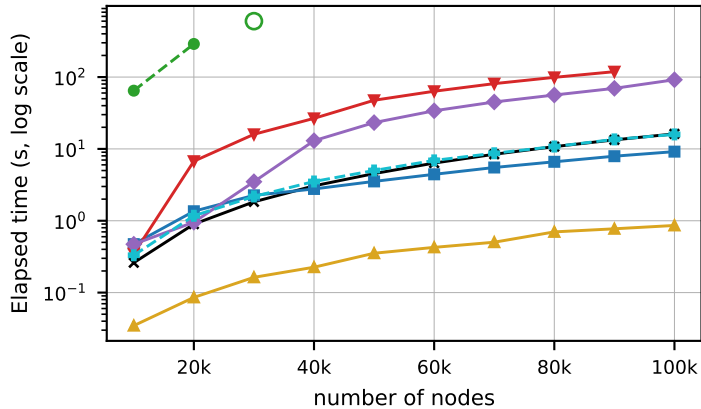
Barabási-Albert: left recursion
