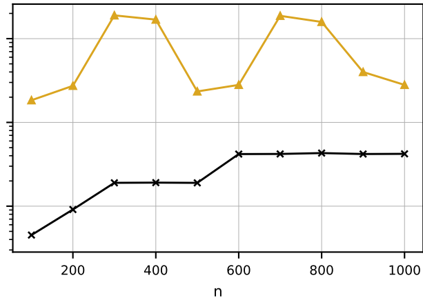
BinTree: right recursion
