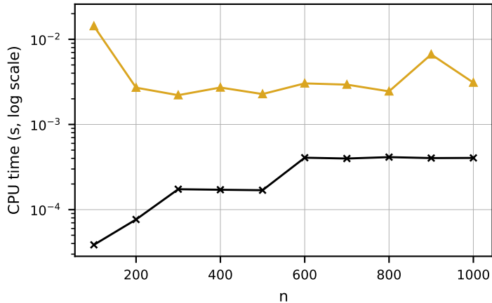
BinTree: left recursion
