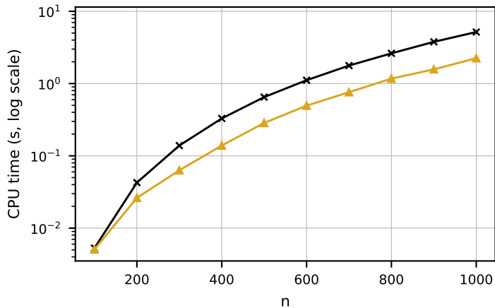
MaxAcyc: left recursion
