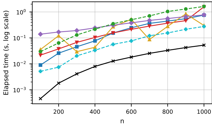
Path: left recursion
