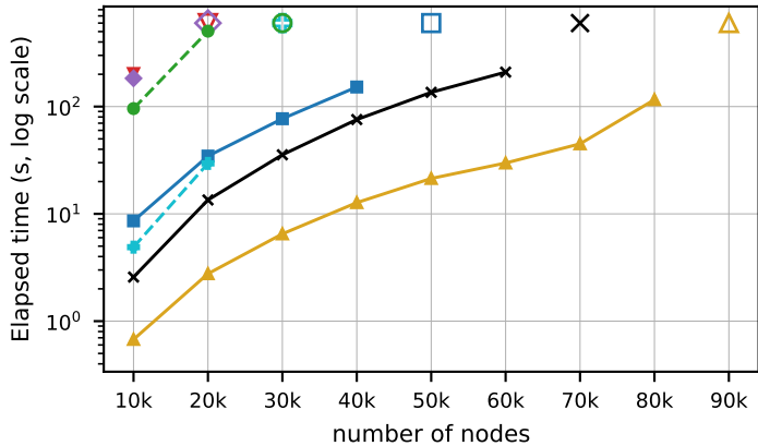
Scale-free: left recursion
