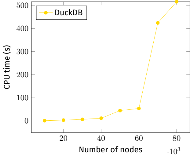
Graph: Scale Free
