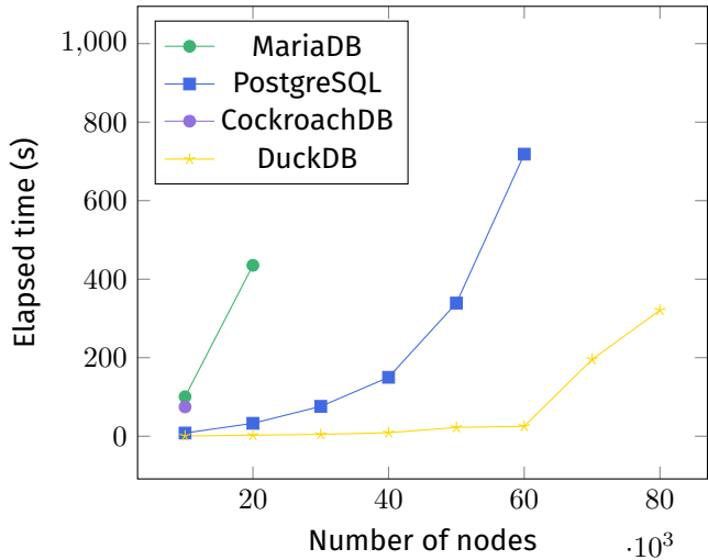
Graph: Scale Free
