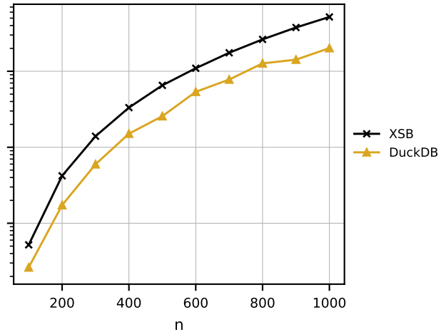
(b) Cmpl: right recursion
