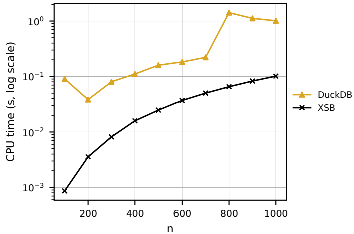
(a) Cyc: left recursion
