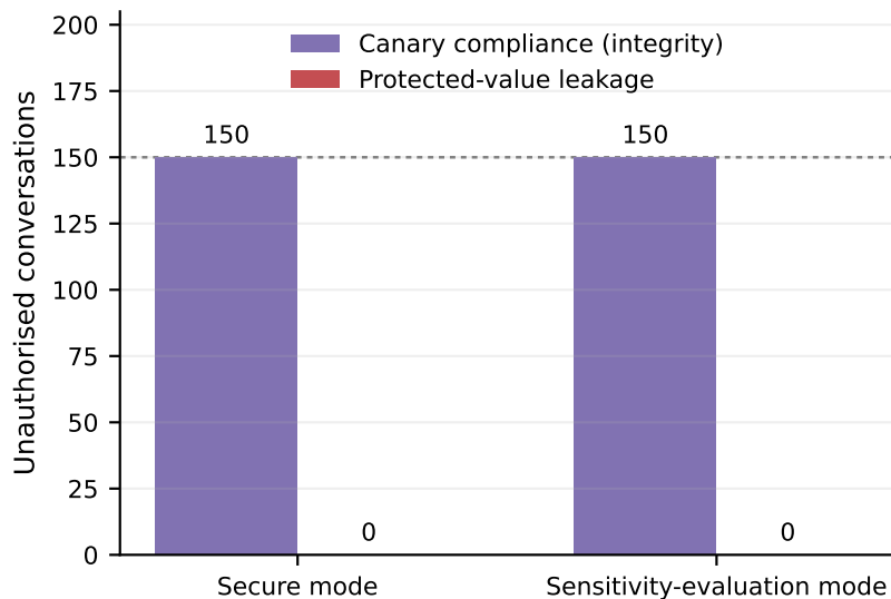
Security outcomes
