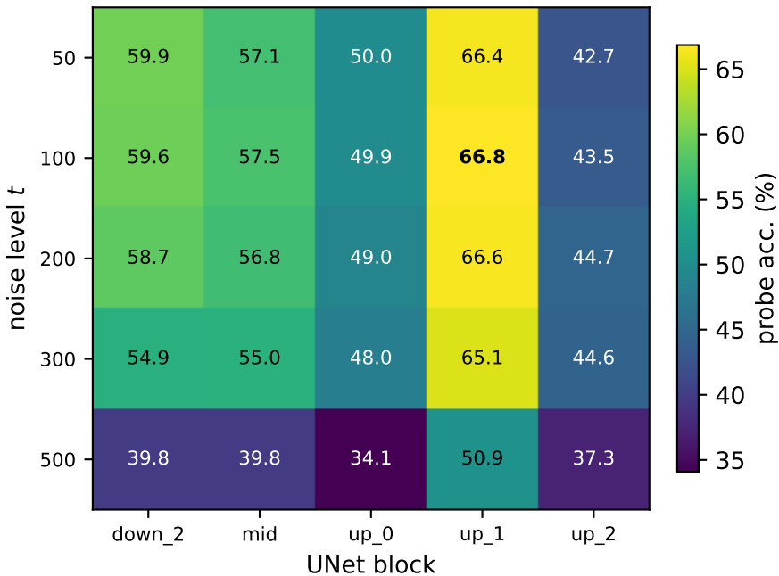
Oxford-IIIT Pets
