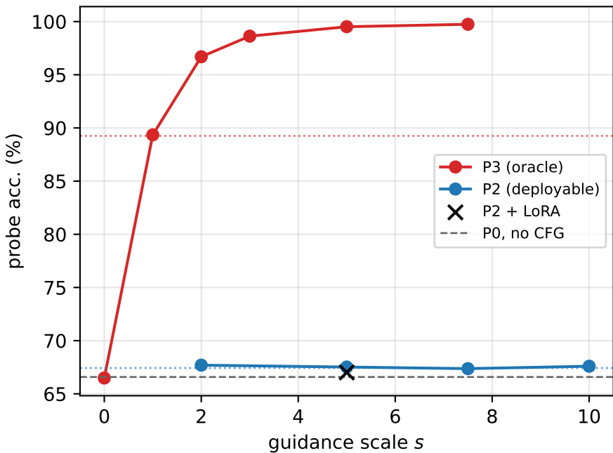
Pets, cfg/up_1, t = 200
