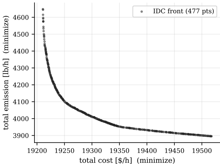
MOEDD13 — cost/emission Pareto front (§8.3)
