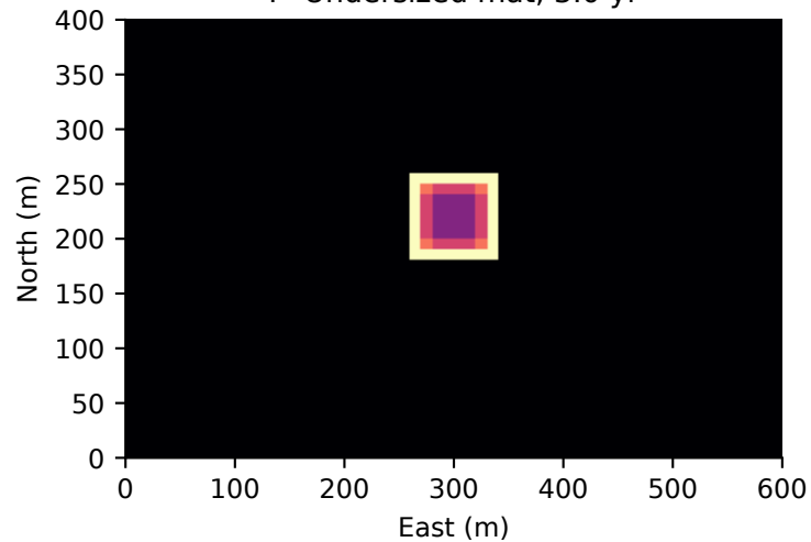
F Undersized mat, 3.0 yr
