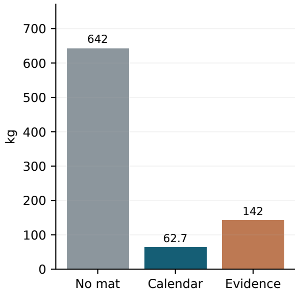
Whole-hotspot Pb emission
