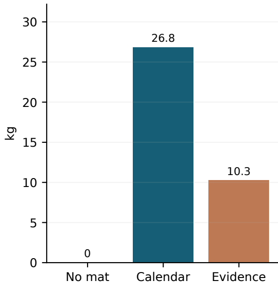
Active + retrieved column Pb
