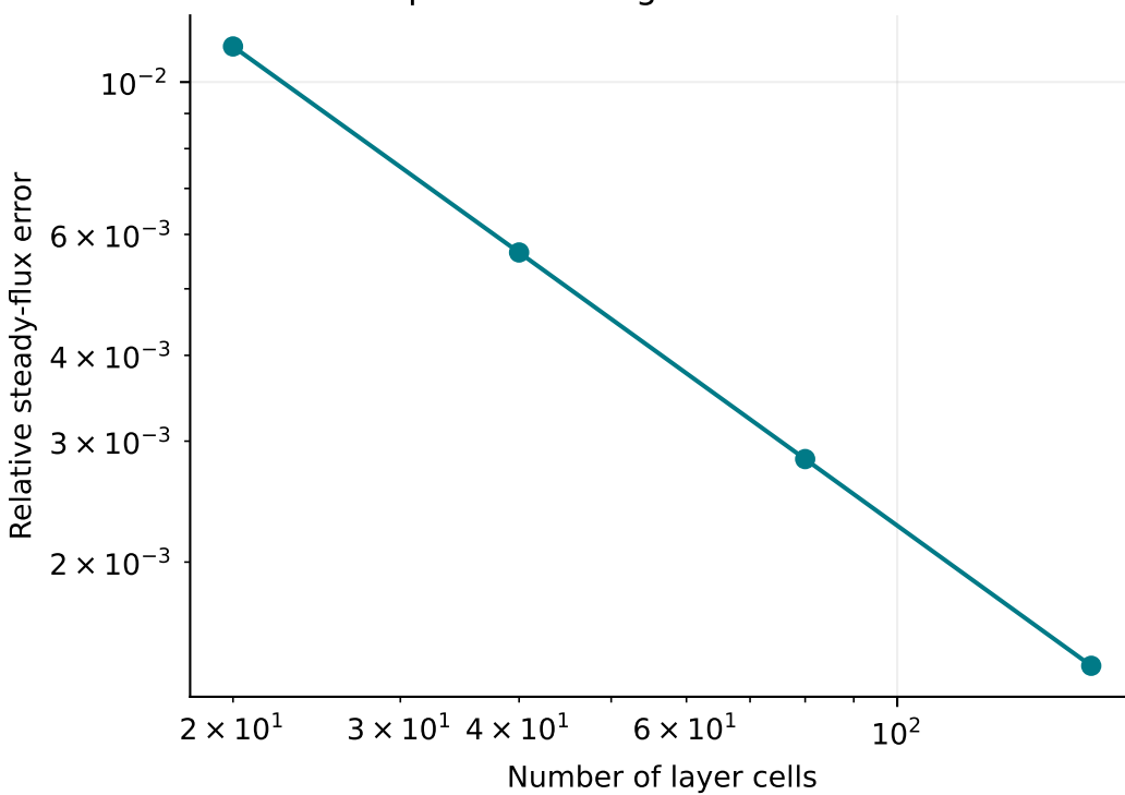
C Spatial convergence to continuum
