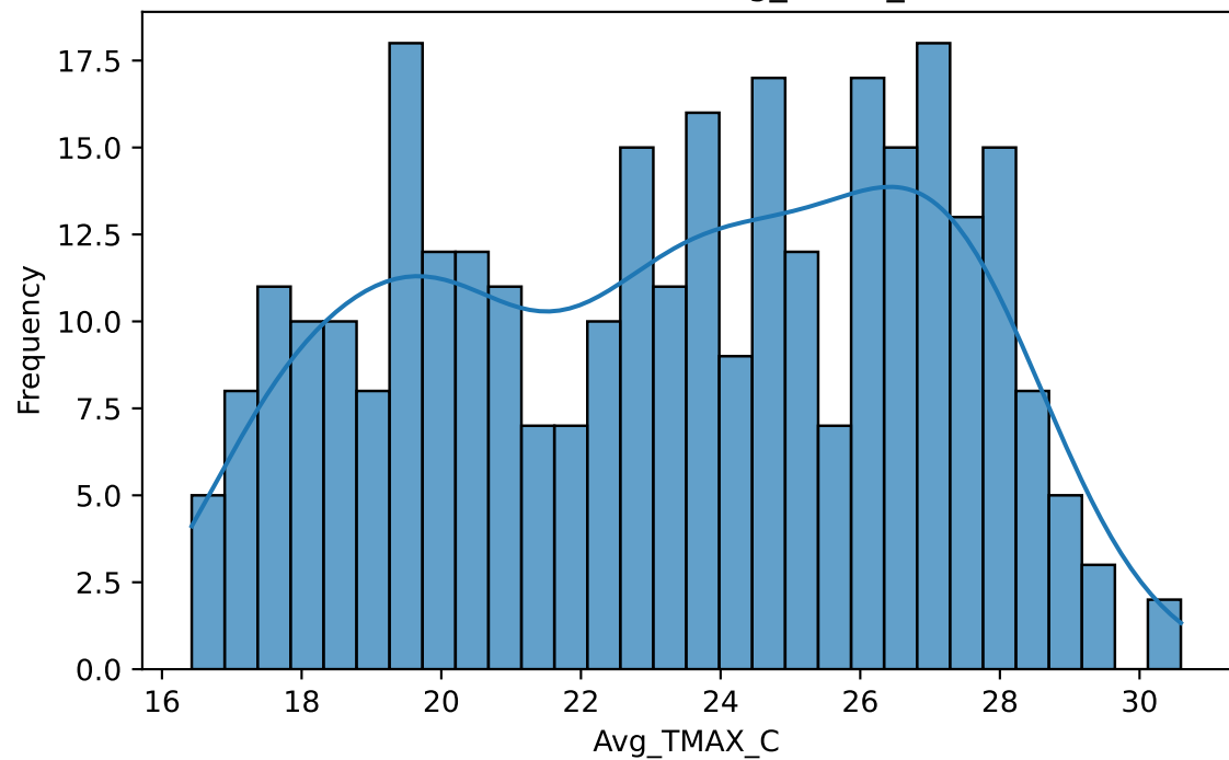
Distribution of Avg_TMAX_C
