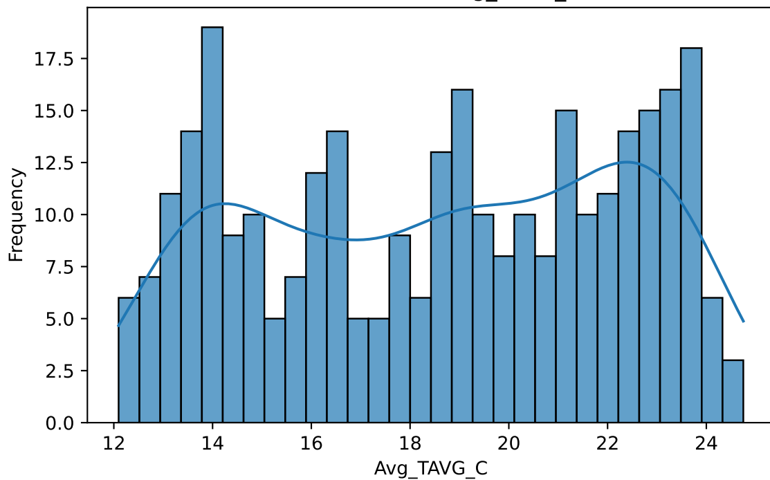
Distribution of Avg_TAVG_C
