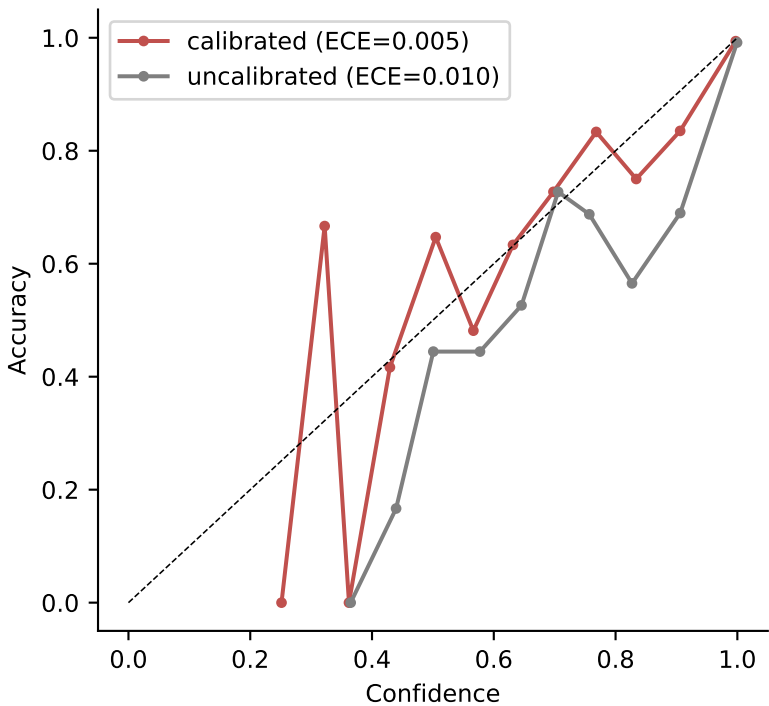
Reliability (multiclass top-class)
