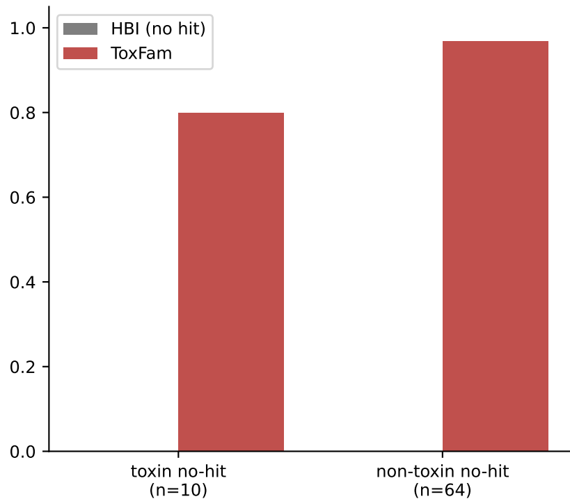
B. No-hit coverage (n=74: HBI 0% by construction)
