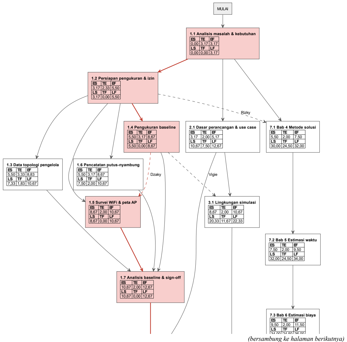
Diagram PERT (activity-on-node) - Jadwal Baseline Opsi B Kotak: ES | TE | EF (atas), LS | TF | LF (bawah); merah muda = rantai kritis; garis putus-putus = ketergantungan sumber daya
