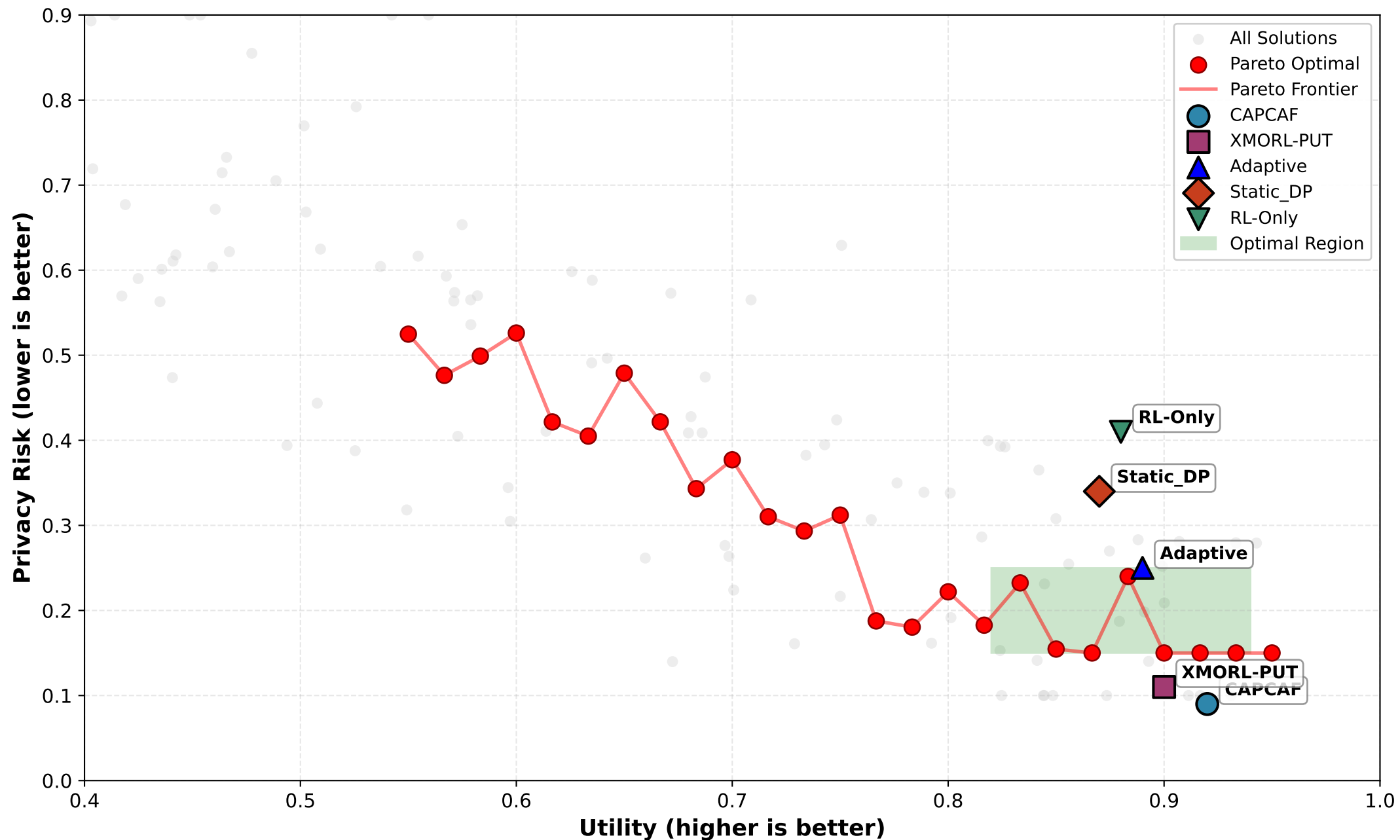
Enhanced Pareto Frontier Analysis with Framework Comparison
