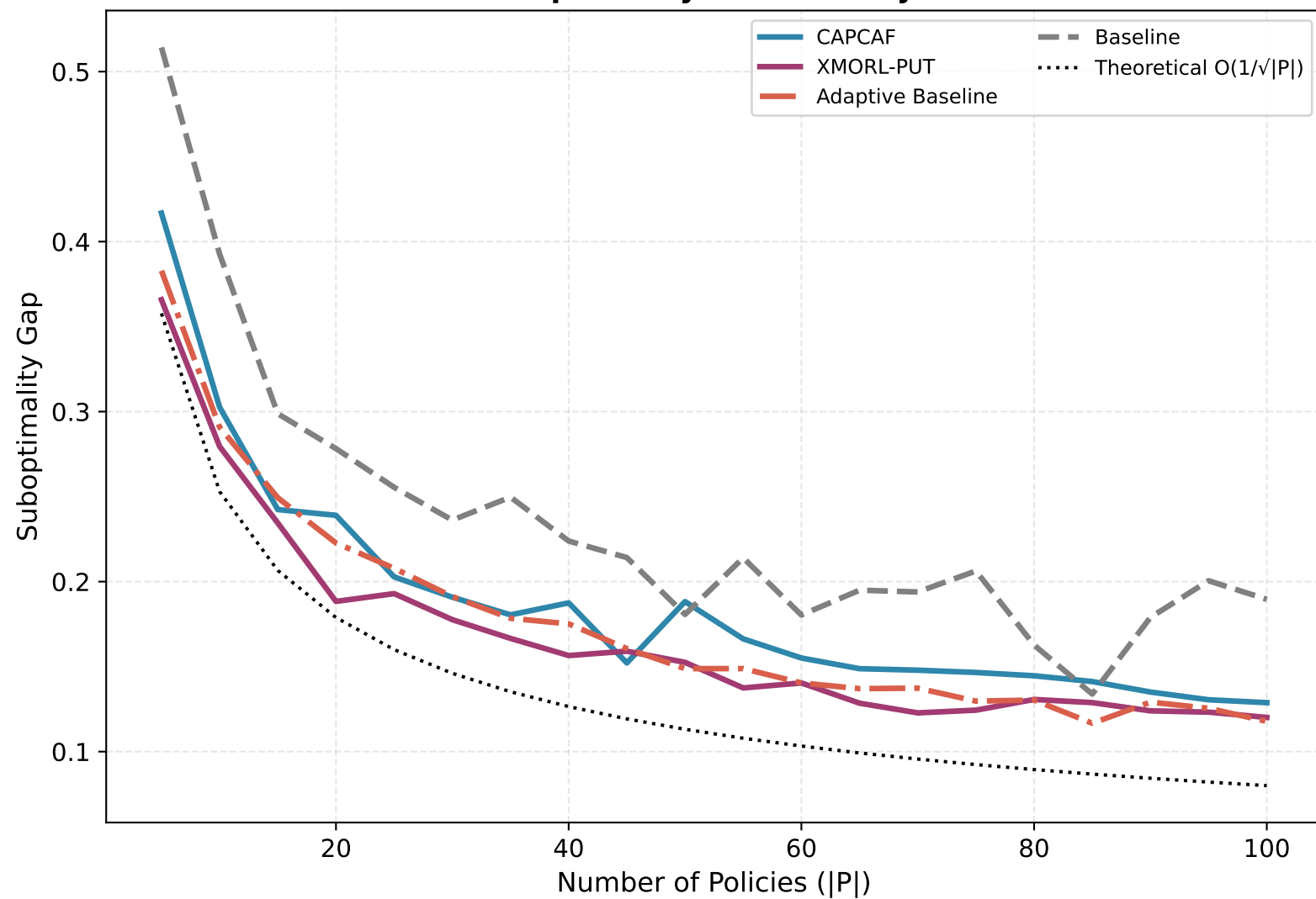
Suboptimality Bound Analysis
