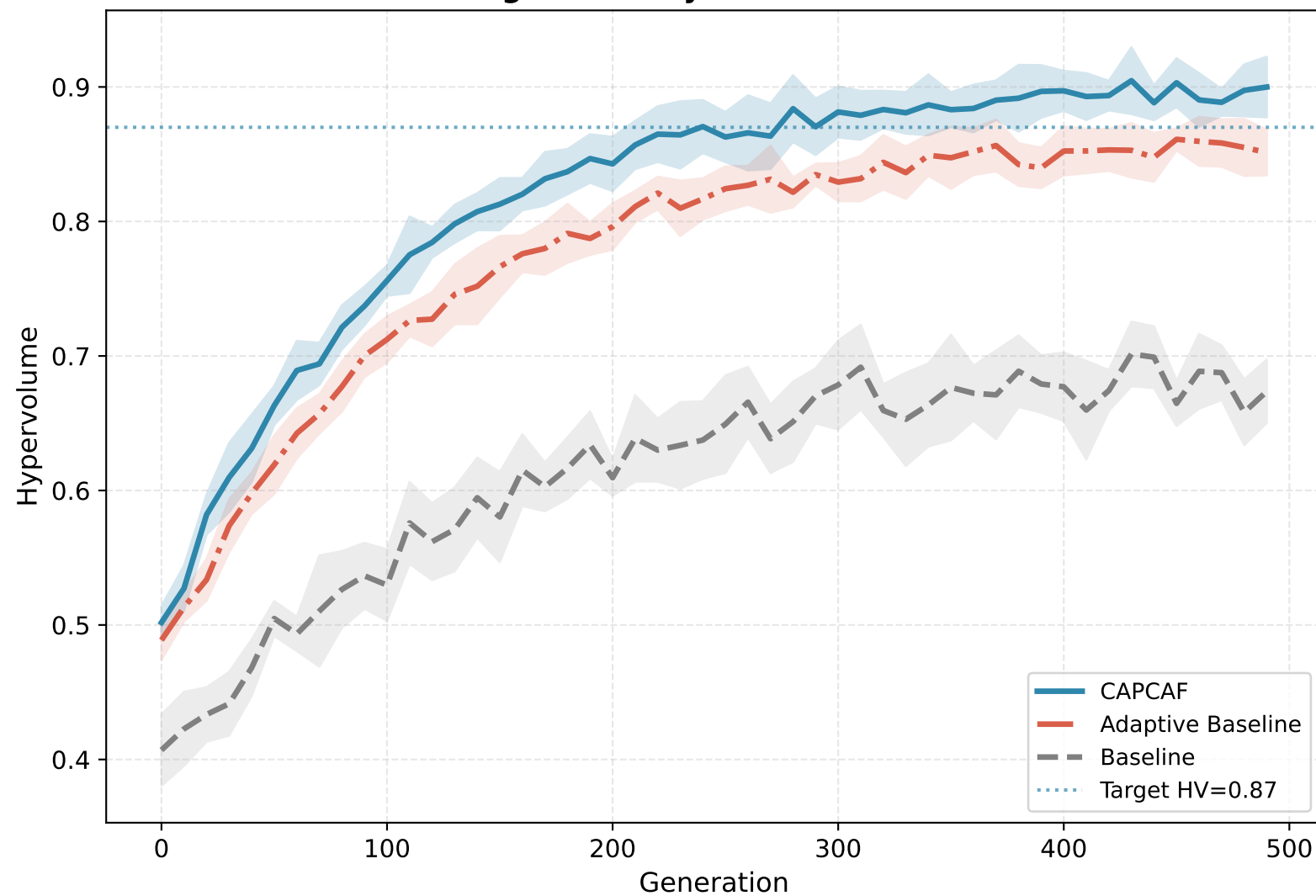
NSGA-II Convergence Analysis with Confidence Intervals
