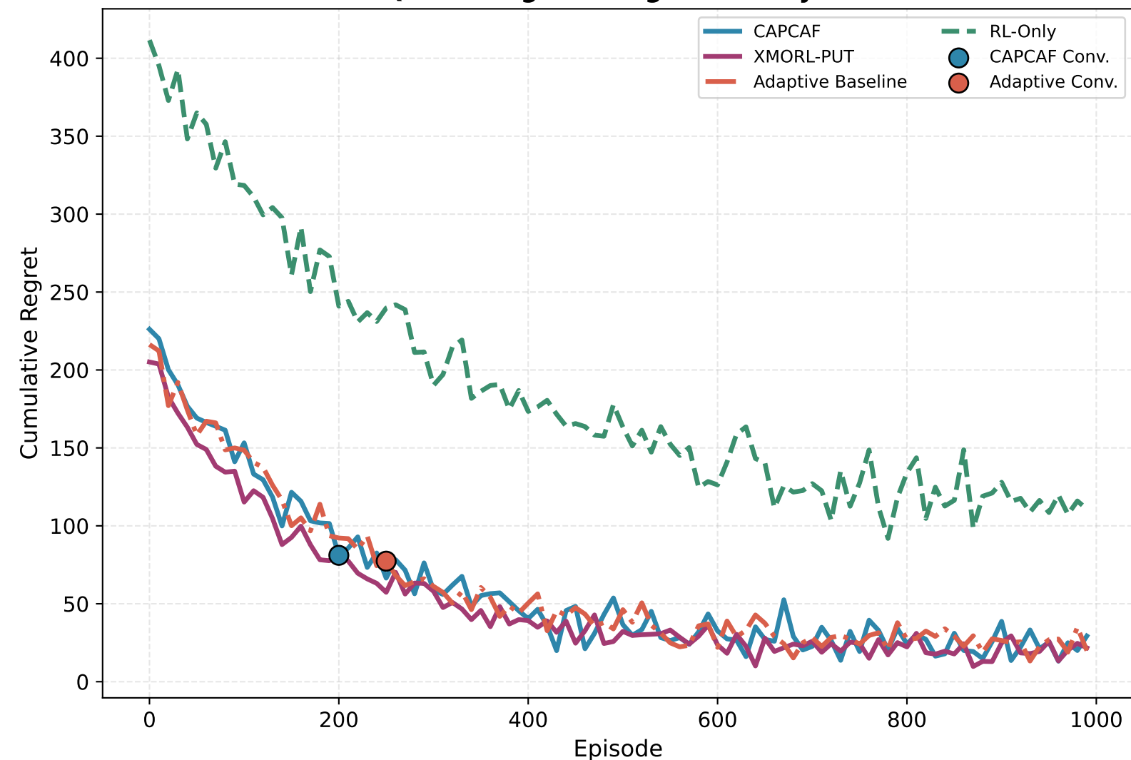
Q-Learning Convergence Analysis
