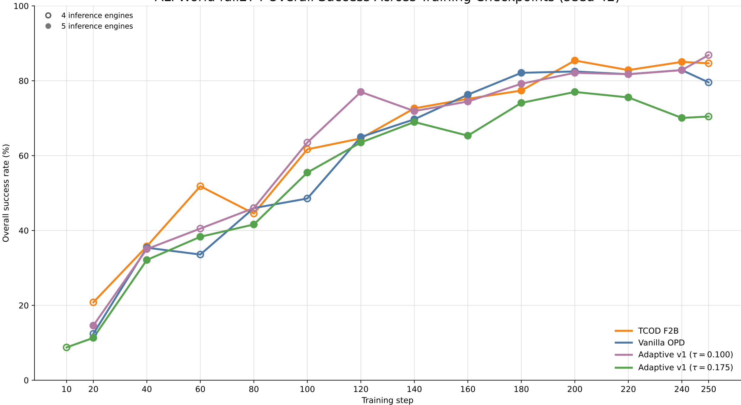
ALFWorld full274 Overall Success Across Training Checkpoints (seed 42)
