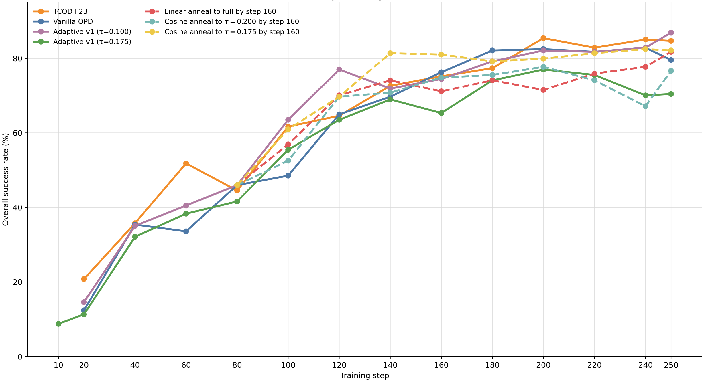
ALFWorld full274: All Training Checkpoint Success Curves (seed 42)
