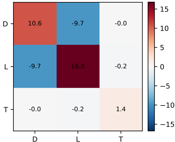
(a) avg within-species block stiff(D-L net growth)=23.9, soft(D+L turnover)=3.4
