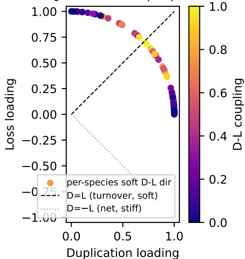
(b) per-species soft D-L direction 29% align w/ turnover, |\cos|_{\text{med}}=0.79
