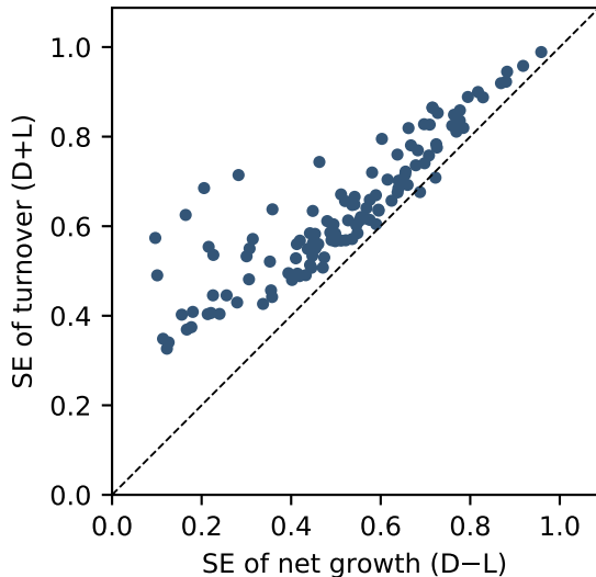
(b) turnover is less identified median var ratio (turn/net)=1.4
