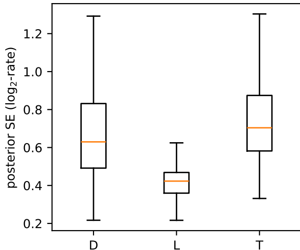
(a) per-rate posterior SE at \lambda=1.0 (MAP cov H_F^{-1} )
