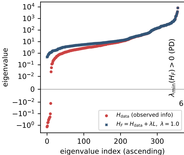
(a) spectrum at the \lambda = 1.0 optimum
