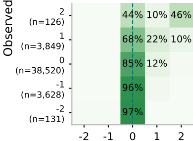
Qwen2.5-72B
