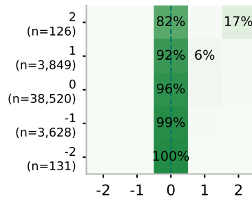
Qwen2.5-32B
