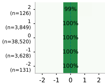
Qwen2.5-7B (4-bit)
