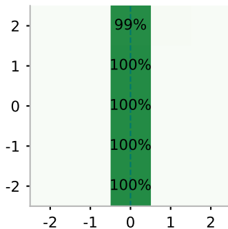
Qwen2.5-7B (4-bit)
