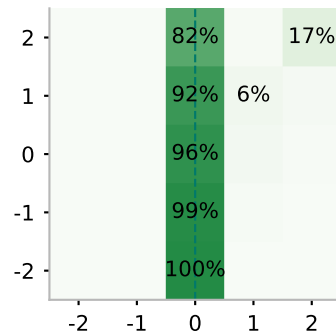
Qwen2.5-32B
