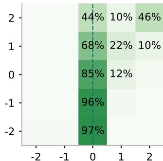
Qwen2.5-72B
