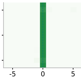
Qwen2.5-32B
