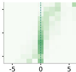
Qwen2.5-72B
