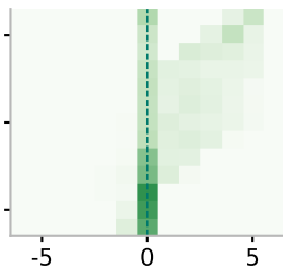
Qwen2.5-7B (4-bit)
