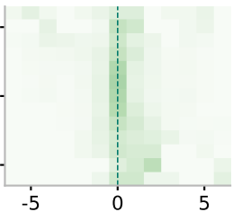
Qwen2.5-7B (4-bit)
