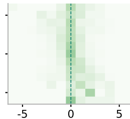
Qwen2.5-72B
