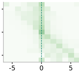
Qwen2.5-32B
