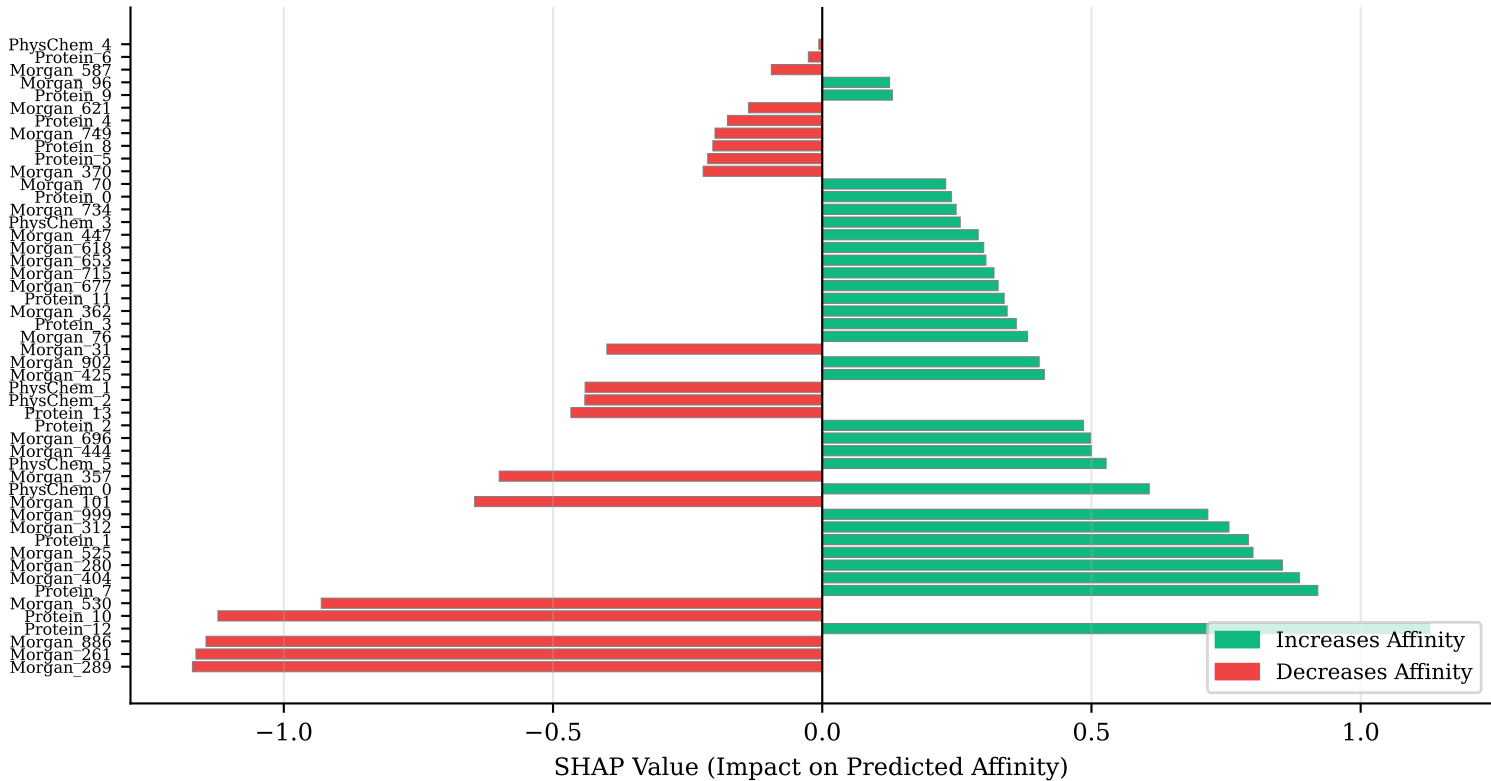
Fig. 4. SHAP Feature Attribution for Top 50 Features
