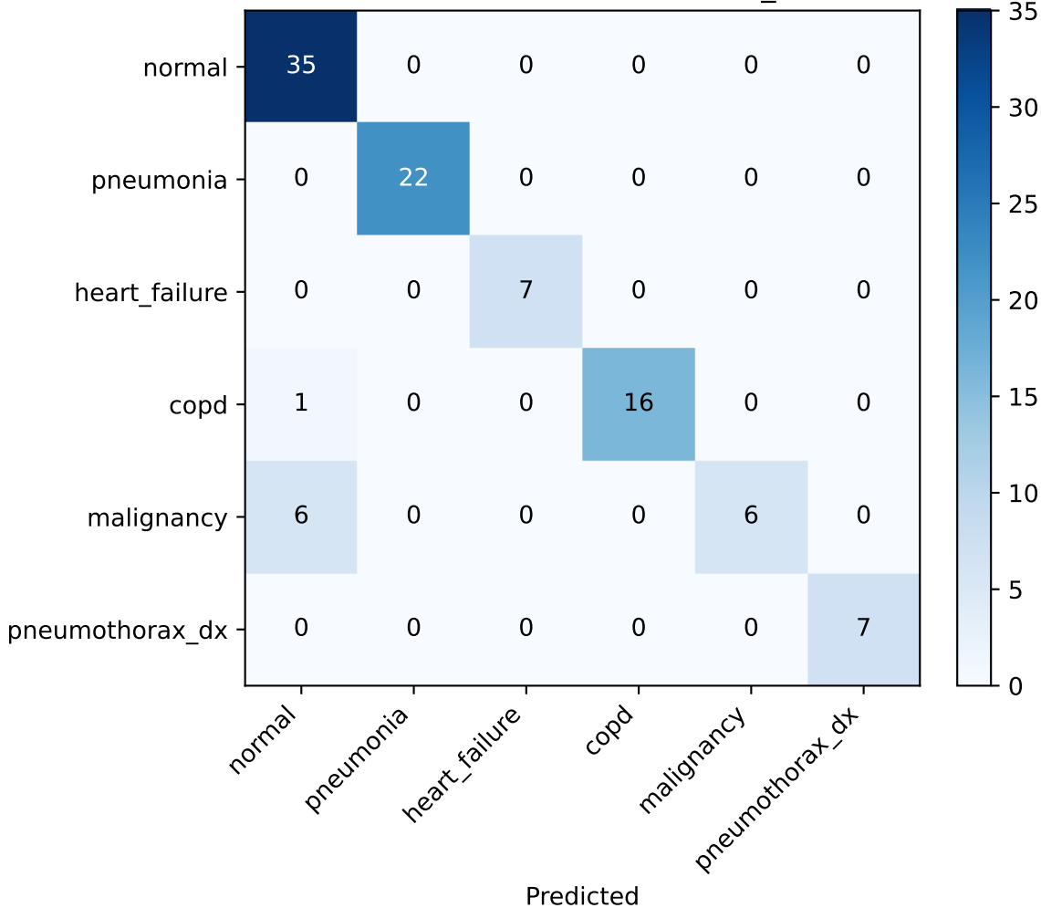
Confusion matrix — classical_fair
