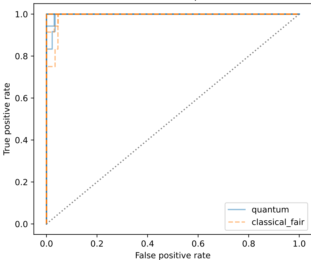
ROC (one-vs-rest, per class)
