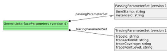
Figure 4 bss.genericInterfaceParameters.response.4 UML representation
