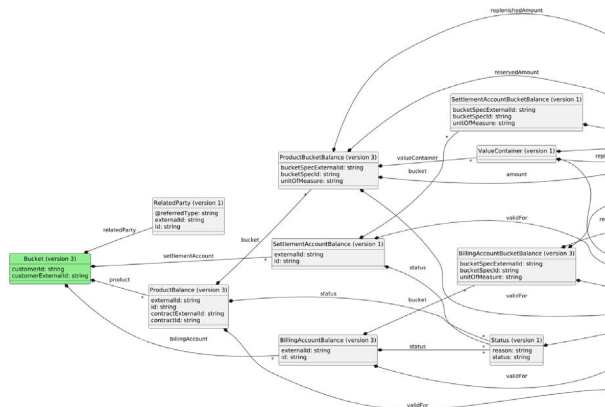
Figure 2 bss.bssfBalanceEnquiry.bucket.readResponse.3 UML representation
