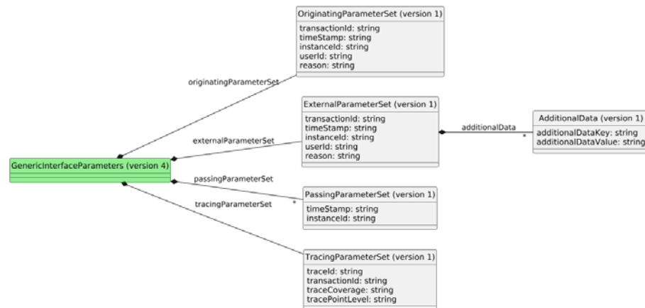
Figure 3 bss.genericInterfaceParameters.request.4 UML representation
