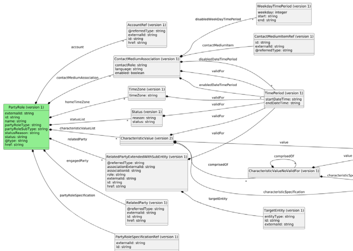
Figure 5 bss.Tmf669PartyRoleManagement.partyRole.updateResponse.1 UML representation
