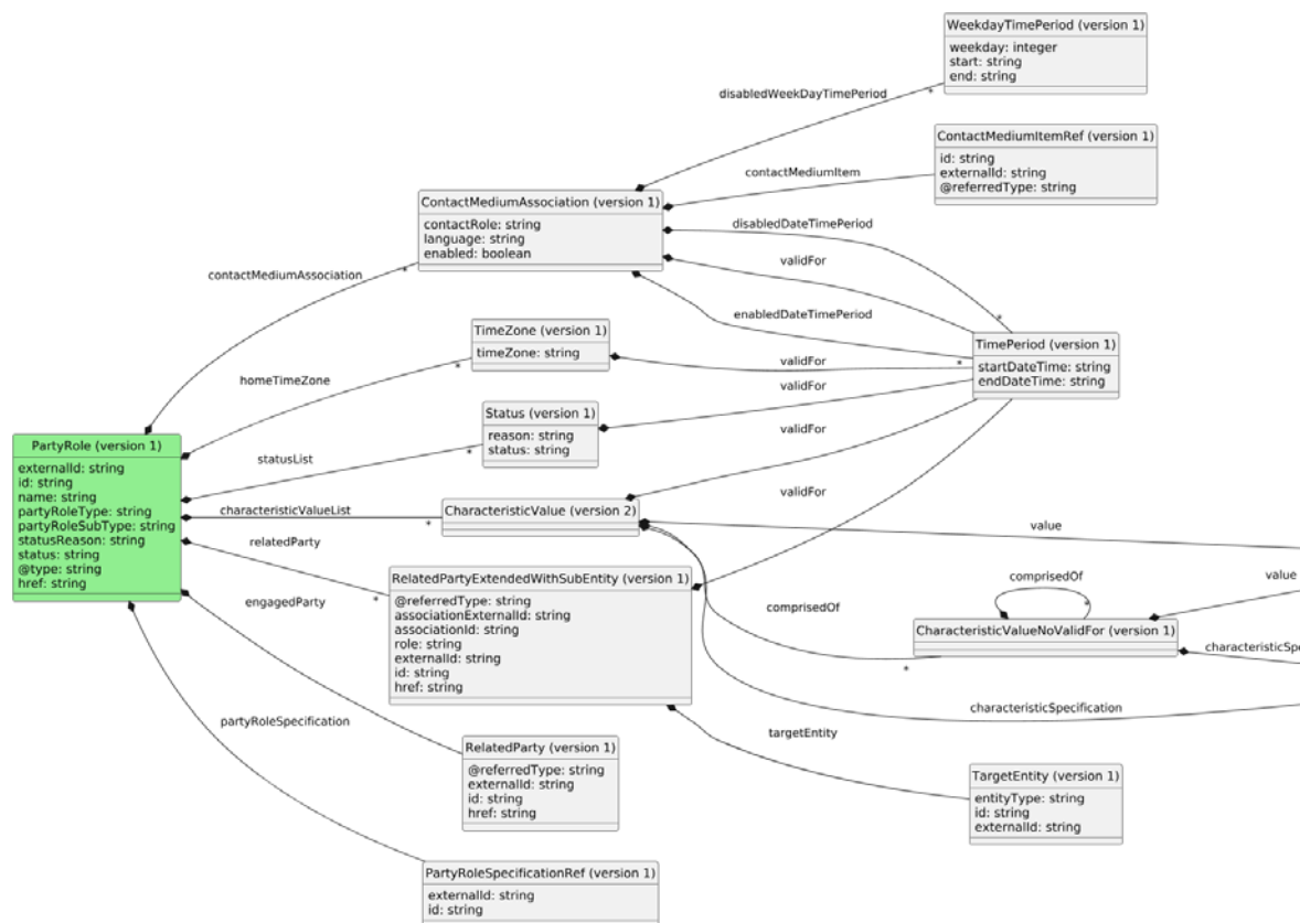
Figure 2 bss.Tmf669PartyRoleManagement.partyRole.createResponse.1 UML representation
