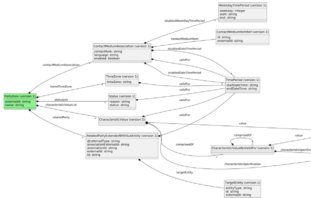
Figure 4 bss.Tmf669PartyRoleManagement.partyRole.updateRequest.1 UML representation
