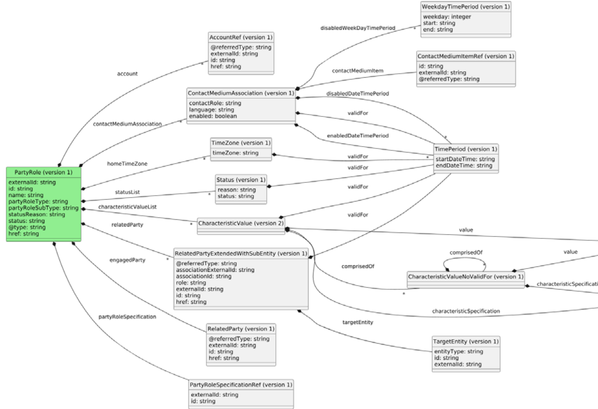
Figure 3 bss.Tmf669PartyRoleManagement.partyRole.readResponse.1 UML representation
