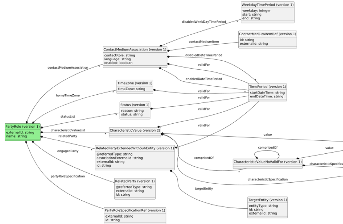
Figure 1 bss.Tmf669PartyRoleManagement.partyRole.createRequest.1 UML representation
