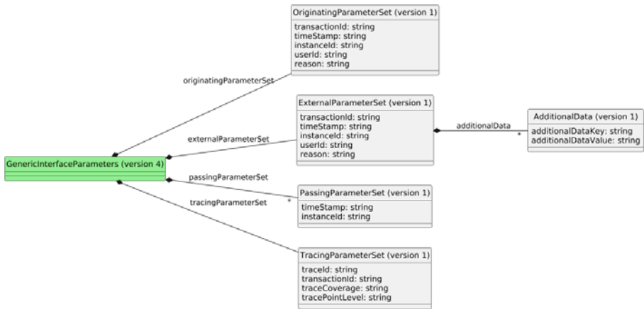
Figure 7 bss.genericInterfaceParameters.request.4 UML representation
