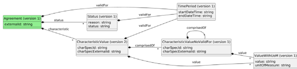
Figure 3 bss.bssfAgreementManagement.agreement.updateRequest.1 UML representation
