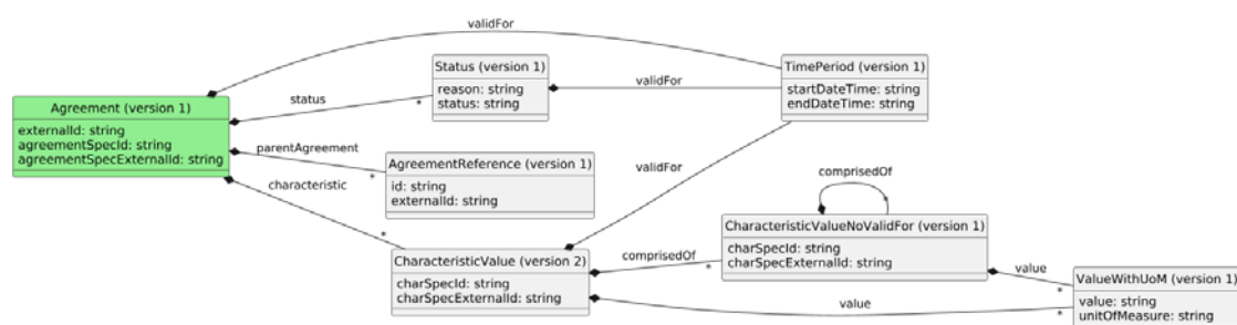
Figure 1 bss.bssfAgreementManagement.agreement.createRequest.1 UML representation
