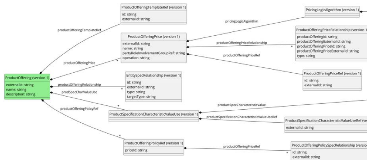
Figure 1 bss.bssfProductCatalogIntegration.productOffering.createRequest.1 UML representation
