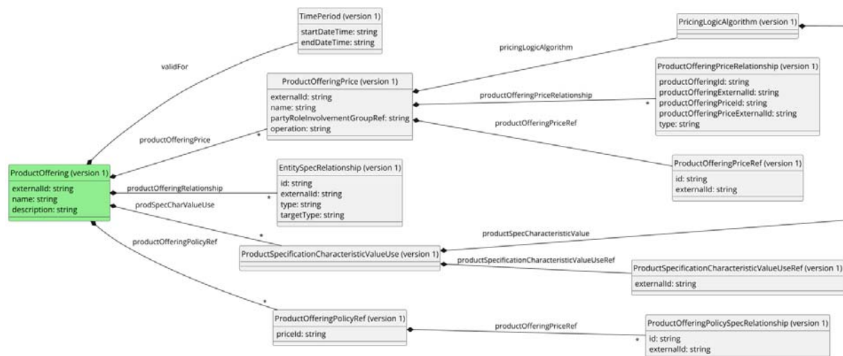
Figure 4 bss.bssfProductCatalogIntegration.productOffering.updateRequest.1 UML representation
