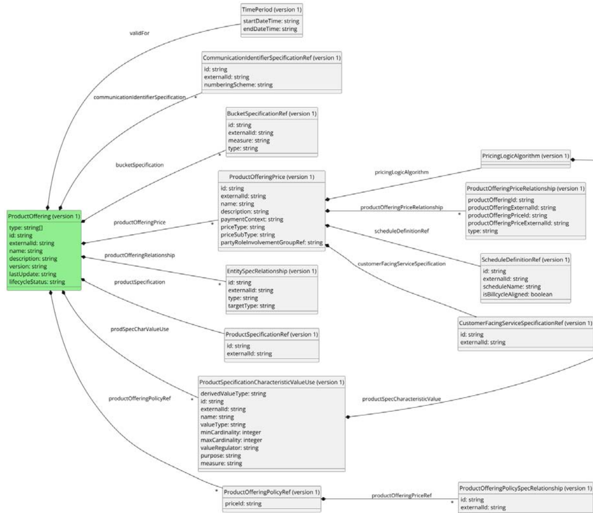
Figure 2 bss.bssfProductCatalogIntegration.productOffering.createResponse.1 UML representation
