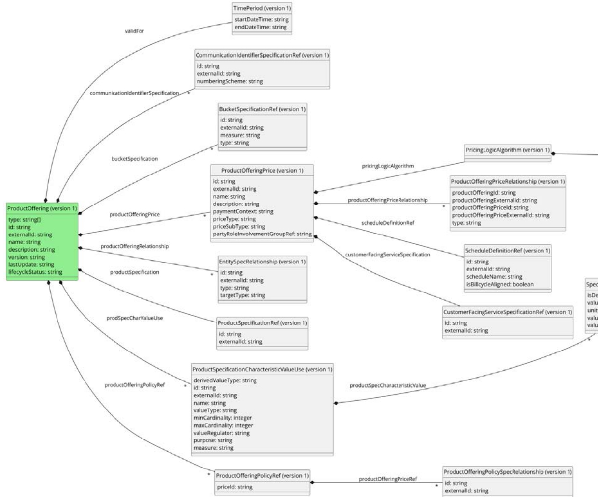
Figure 5 bss.bssfProductCatalogIntegration.productOffering.updateResponse.1 UML representation
