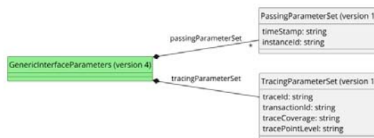
Figure 7 bss.genericInterfaceParameters.response.4 UML representation
