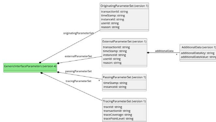
Figure 6 bss.genericInterfaceParameters.request.4 UML representation
