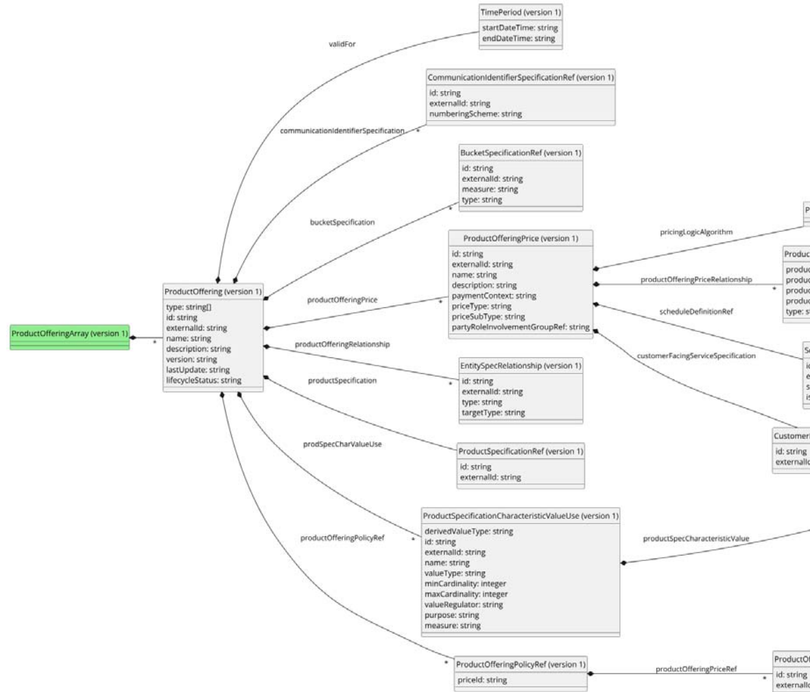
Figure 3 bss.bssfProductCatalogIntegration.productOffering.readResponse.1 UML representation
