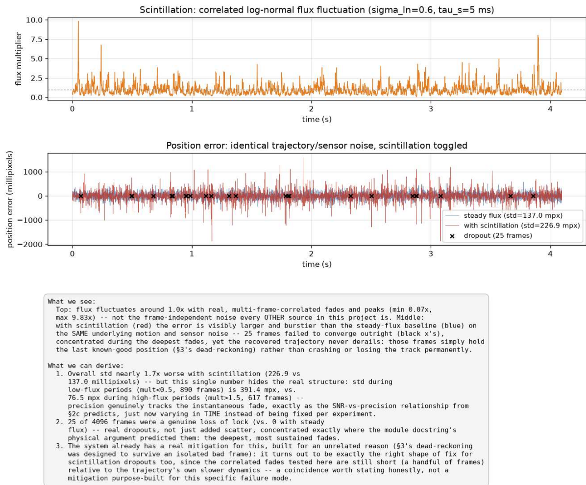
Figure 7: position error under atmospheric scintillation, steady flux vs. correlated fading.
