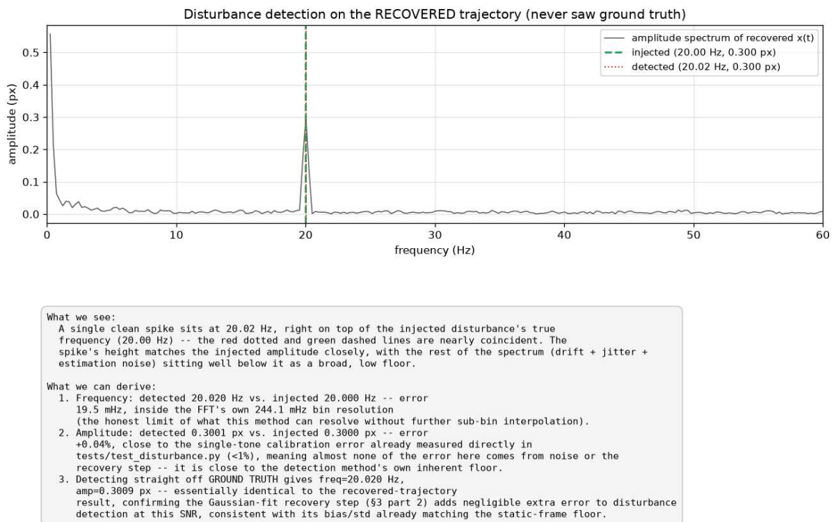
Figure 5: recovered versus injected disturbance frequency and amplitude.
