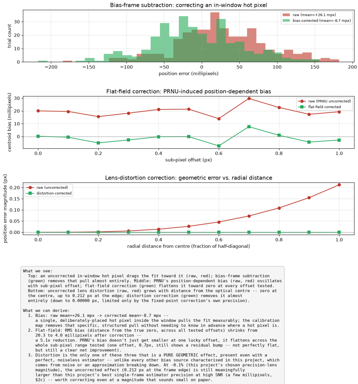
Figure 13: Figure 12: measured effect of bias, flat-field, and distortion calibration on position bias.
