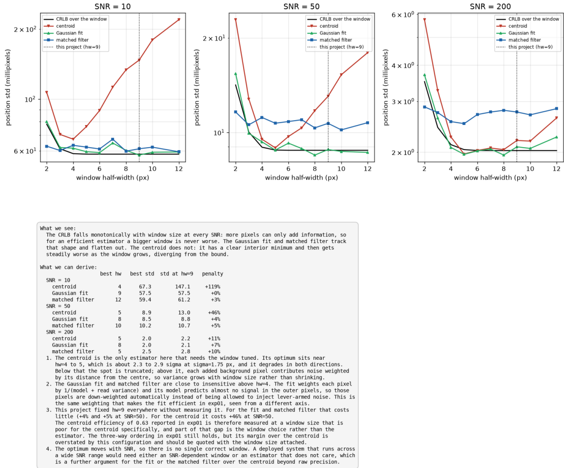
Figure 18: Figure 17: estimator precision versus window half-width against the CRLB, at three SNR levels.
