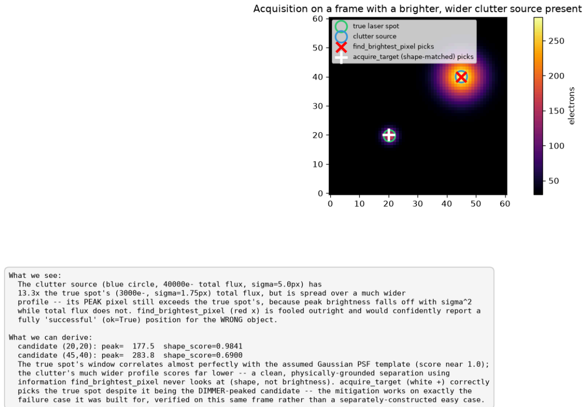
Figure 9: Figure 8: acquisition on an identical frame containing a bright clutter source, brightest-pixel versus shape-matched.
