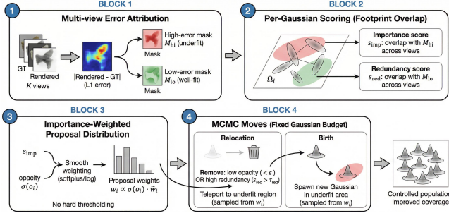
Figure 4: We aggregate multi-view reconstruction errors into per-Gaussian importance and redundancy scores, then use the resulting importance-weighted distribution for both relocation and birth. This reallocates model capacity toward persistently underfit regions while preserving the underlying MCMC population-management framework.
