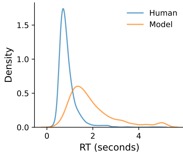
Stimulus 5 (n=1485) Model: \mu=1.929s , \sigma=1.020s Human: \mu=0.983s , \sigma=0.423s
