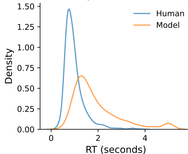
Stimulus 7 (n=1539) Model: \mu=1.914s , \sigma=1.010s Human: \mu=0.977s , \sigma=0.439s
