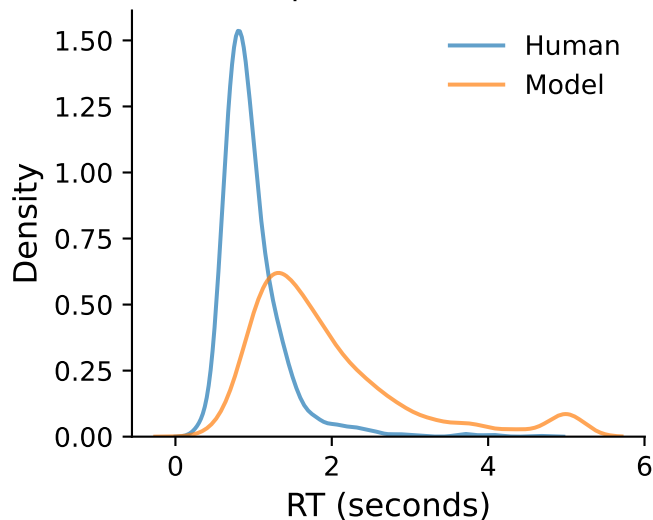
Stimulus 5 (n=1485) Model: \mu=1.929s , \sigma=1.020s Human: \mu=0.983s , \sigma=0.423s
