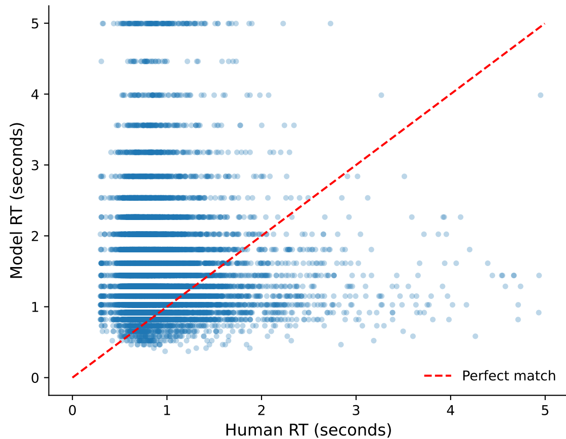
A. RT Correlation ( r=-0.005 )
