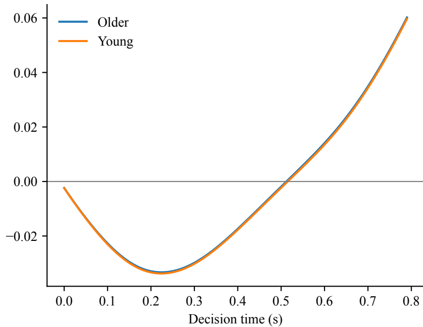
Target minus flanker S(t)
